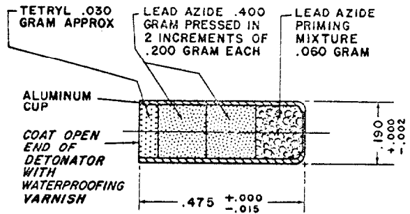
DETONATOR MK 28 MOD O
